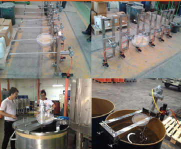
AIR MIXER
